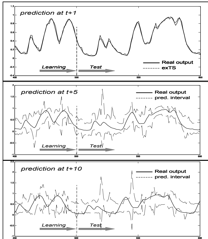
Figure 4. Accuracy of predictions and prediction intervals (95% confidence).
