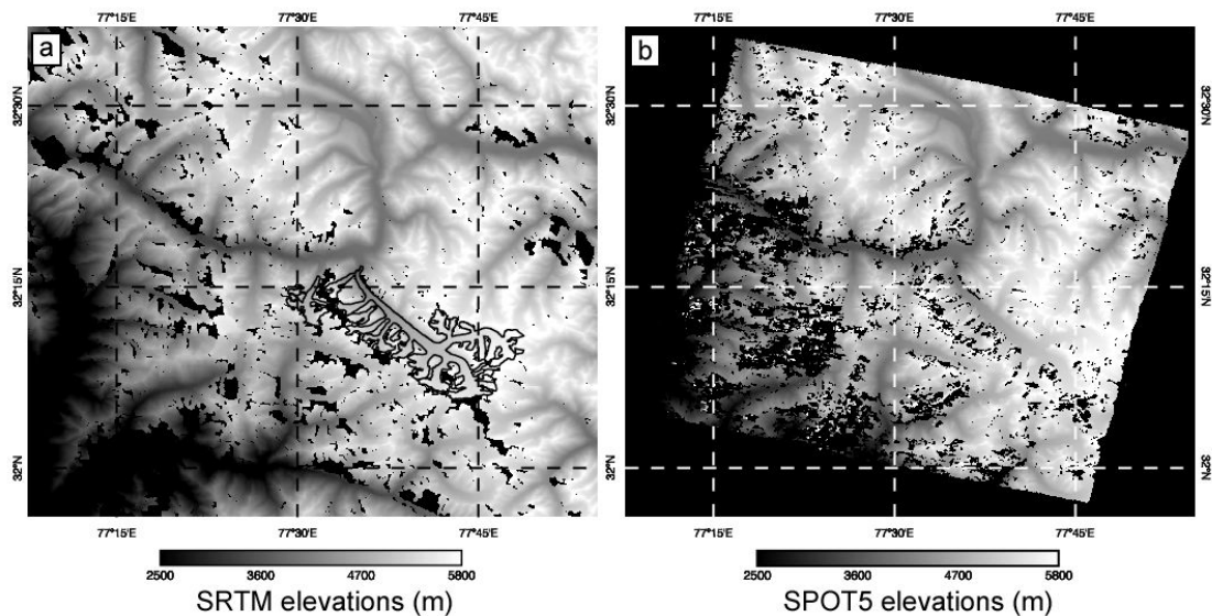
Figure 4: SRTM (a) and SPOT5 (b) DEMs. The boundaries of the Chhota Shigri (16.5 km 2 ) and the Bara Shigri (133 km 2 ) glaciers are overlaid in dark on the SRTM-DEM.
