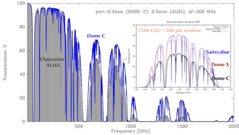
Fig. 2. Modelled transmission for Dome C and Chajnantor/ALMA site with the MOLIÈRE code. Transmissions were estimated using PWV=0.2 mm for Dome C (blue) and 0.5 mm for ALMA site (grey) that represent the expected first quartile PWV values. 200- \mu\text{m} (1500 GHz) windows open at Dome C. Note: MOLIÈRE (Microwave Observation Line Estimation and REtrieval) is a versatile forward and inversion model for the millimetre and submillimetre wavelengths range, used in many aeronomy and some astronomy applications (Urban 2004). Plots produced by N. Schneider-Bontemps. Inset plot with am code shows the comparison of the 200- \mu\text{m} transmission for PWV=0.1 mm at Dome C, at Sairecabur (a 5525-m Chilean site) and Dome X, a fictive site with atmospheric profile as Dome C but at a pressure altitude of 5525 m. The Chilean site has the highest transmission. At equal altitudes and pressures, Chilean site vs. Dome X, Chilean site would win over Antarctica lower temperature conditions. This is because low temperatures bias \text{H}_2\text{O} partition function and strengthen THz absorption lines. Comparing Dome C with Sairecabur, higher atmospheric pressure at Dome C broadens very strong lines that bound THz windows. Overall: the transmission for PWV=0.2 mm at Dome C is comparable to the transmission for PWV=0.35 mm at 5500m in Chile. However, this comparison does not take into account the percentiles of PWV at both sites and need to be confirmed by observations. The models were done with the am modeling software: http://sma-www.cfa.harvard.edu/private/memos/152-03.pdf . Plots produced by D. Marrone
