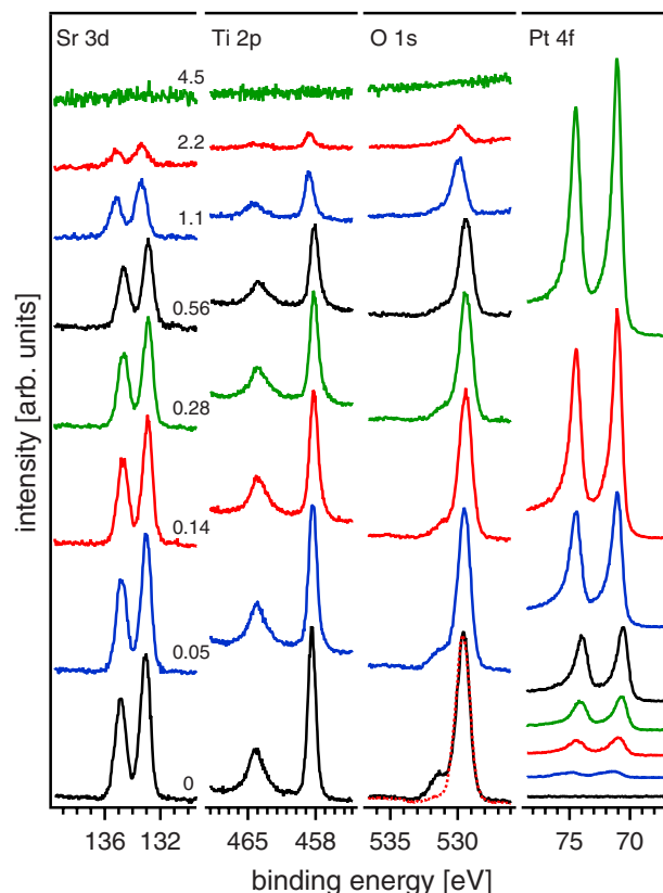
FIG. 3. (Color online) X-ray photoelectron spectra recorded during stepwise deposition of Pt onto Ba 0.6 Sr 0.4 TiO 3 . The Pt film thickness is indicated in nanometers. All of the spectra were recorded by using monochromatic Al K \alpha radiation and referenced to the Fermi edge of a sputter cleaned Ag sample. The O 1 s spectrum of a BST film deposited under conditions which lead to a Ti excess is given as a dotted line.
