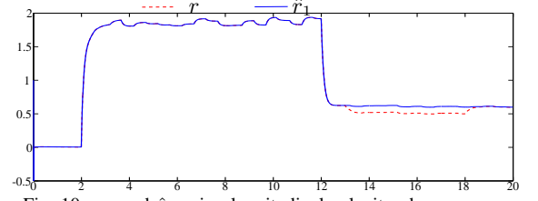
Fig. 10. r and \hat{r}_1 using longitudinal velocity observer 1
