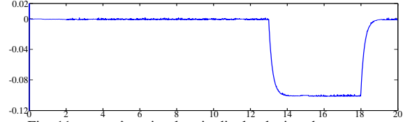
Fig. 11. r - \hat{r}_1 using longitudinal velocity observer 1
