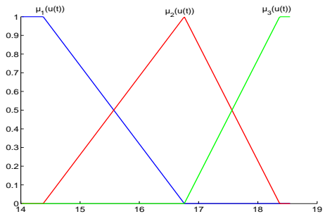
Fig. 1. Membership functions
