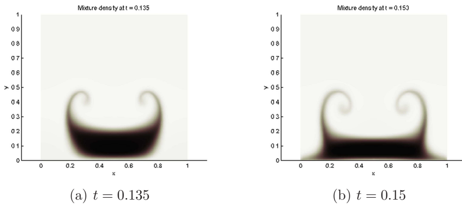
Fig. 17. Water drop test case. Drop/bottom compressible interaction.
