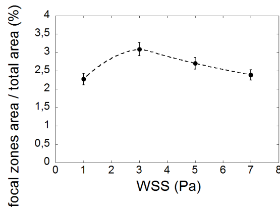
Fig. 14 Area fraction occupied by focal zones on adherent cells in microchannels ( w = 1\text{ mm} , h = 231\ \mu\text{m} ) vs. maximum shear stress experienced. The flow rate, increased every 5 minutes, has generated an increasing wall shear stress: 35, 33, 24 and 31 cells were submitted to a shear stress until 1, 3, 5 and 7 Pa respectively. The dashed line guides the eye. Error bars are standard errors to the mean.
