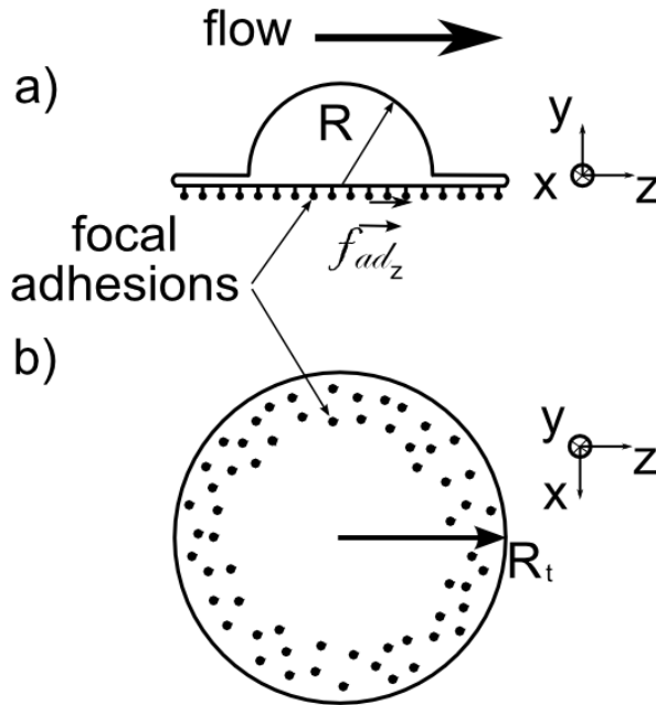
Fig. 17 Schematic views of a cell adhering to a flat surface submitted to a shear flow (flow is from left to right). a) Side view: the cell is modeled as a half-sphere (radius R ), with a circular lamellipodium (radius R_t ). An adhesive force along z with magnitude f_{ad_z} is applied to each one of the N focal adhesion sites. b) Bottom view: dots represent focal adhesion sites, where the individual forces are exerted.
