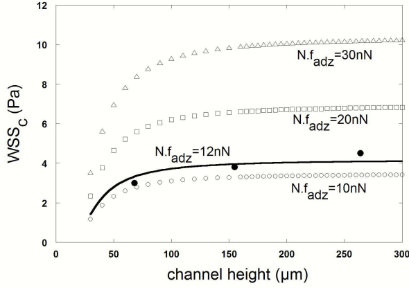
Fig. 18 WSS_c versus h calculated with equation (10) for different values of the Nf_{adz} parameter. R = 15 \text{ }\mu\text{m} . Also shown are the data points and the best fit leading to Nf_{adz} = 12 \text{ nN} .
