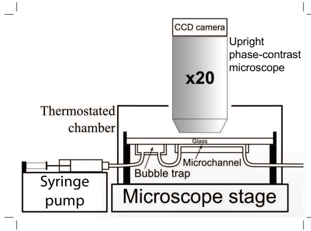
Fig. 1 Full view of the experimental set-up. The microfluidic device is placed in a thermostated chamber at 37° C under the x20 objective of an up-right phase contrast microscope. Fluid flow is controlled by a syringe-pump. Before reaching the microchannel, the fluid first passes through the bubble trap (completely filled with medium before the experiment), where bubbles remain trapped.
