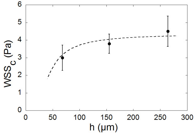
Fig. 12 WSS_c vs. channel height h (at constant w = 1 \text{ mm} ). Data are the mean of the WSS_c measured for all the cells tested in the experiments (10, 5 and 6 cells for the channels with average heights 68, 155 and 264 \mu\text{m} respectively). The dashed lines are the fit of the results based on the model presented in the discussion: experimental values (black dots) are fitted with the hypothesis of equilibrium between adhesion and hydrodynamic forces: F_{flow} = F_{adh} . Results of the fit give : Nf_{adh} = 12 \text{ nN} . Error bars are standard errors to the mean.
