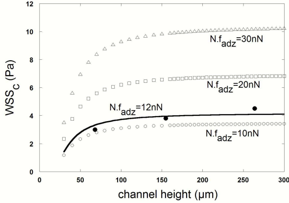
Fig. 18 WSS_c versus h calculated with equation (10) for different values of the Nf_{adz} parameter. R = 15 \mu\text{m} . Also shown are the data points and the best fit leading to Nf_{adz} = 12 \text{ nN} .
