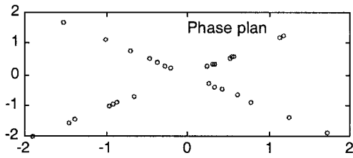
Figure 2c. Phase portrait y(k), y(k-1)
