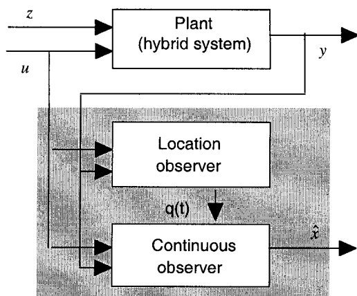
Figure 3. Observer structure
