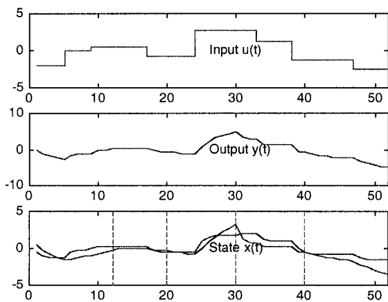
Figure 4. Input, output and state
