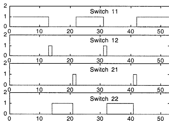
Figure 6. Switching
