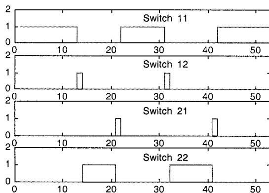
Figure 6. Switching
