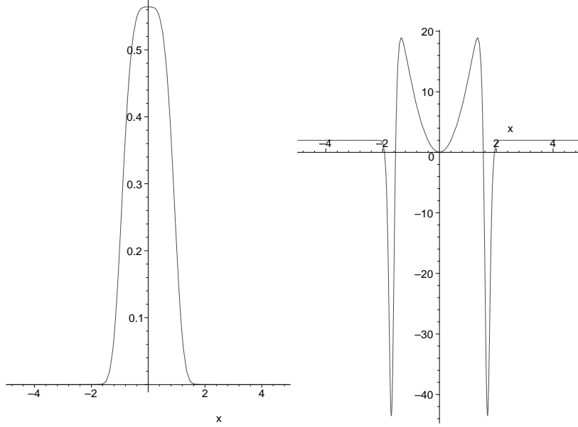
Figure 1: Density and second derivative of -\log -density of \mu_p for Example 4.5.5 with p = 1/100 and a = 4 . The second plot reveals a deep multiple wells potential.
