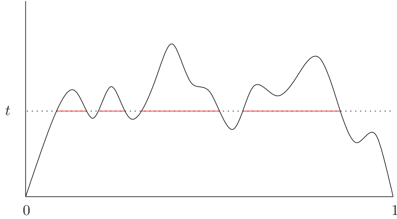
Figure 1: An interval fragmentation derived from a continuous excursion: the set O(t) is represented by the solid lines at level t .
