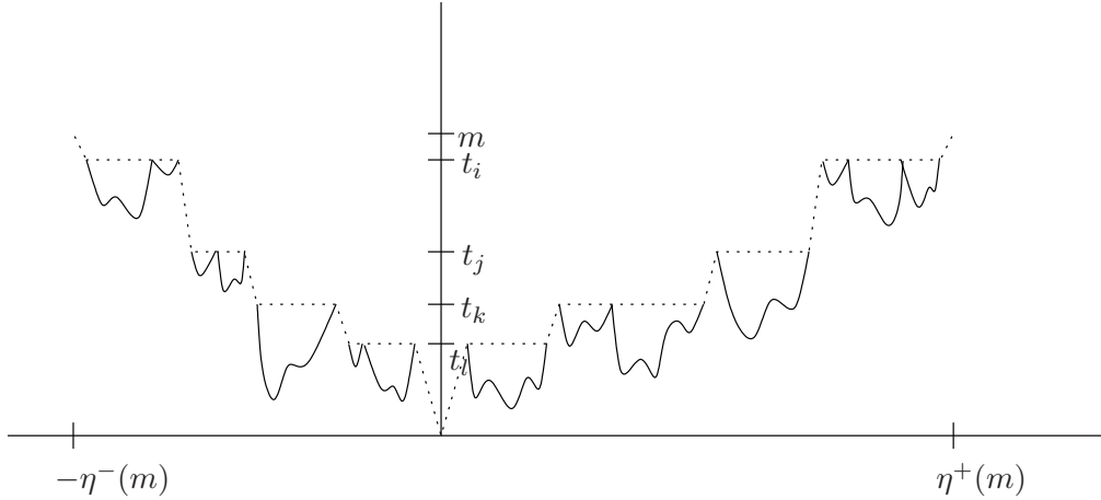
Figure 3: Schematic drawing of H_\infty , with the one-sided running suprema indicated by dotted lines.
