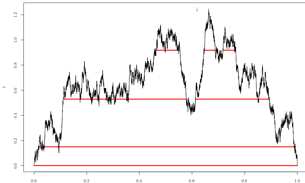
Figure 2: The Brownian interval fragmentation with the open intervals which constitute the state at times t = 0, 0.15, 0.53 and 0.92 indicated.
