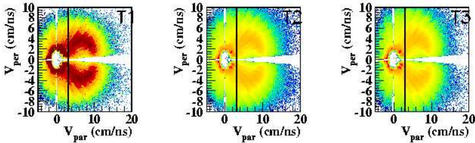
Fig. 3. Invariant velocity diagrams V_{per} versus V_{par} for protons of the regions T1, T2 and T3.
