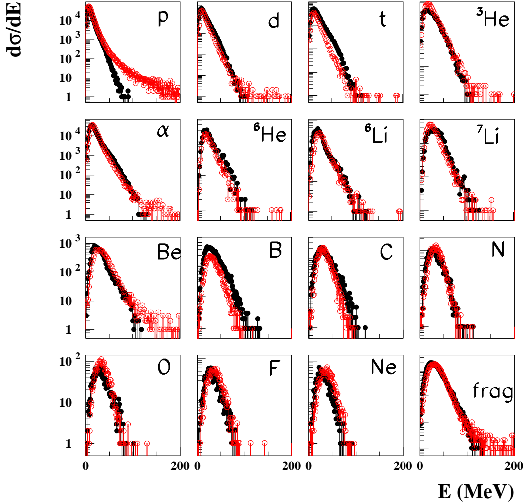
Fig. 4. Backward(black circles)-forward(open circles) energy spectra in the source reference frame of the region T1 for different nuclear species ranging from protons to fragments ( Z > 10 ).
