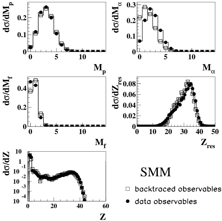
Fig. 8. Comparison between data (points) and SMM results (squares) for region T3. In the top row : M_p : proton multiplicity and M_\alpha : alpha multiplicity; in the middle row : M_f : fragment multiplicity and the residue charge distribution. In the bottom row: the total charge distribution.
