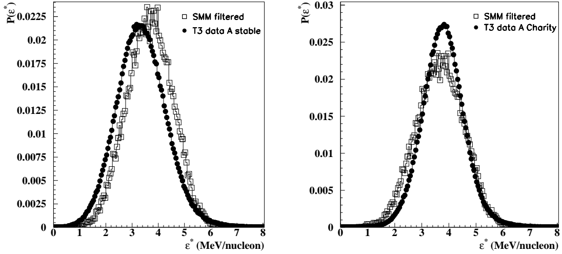
Fig. 10. Source excitation energy for A_{stable} (left) and A_{Charity} (right) mass parameterization. SMM backtraced (open squares) and data excitation energy (full points). Region T3.
