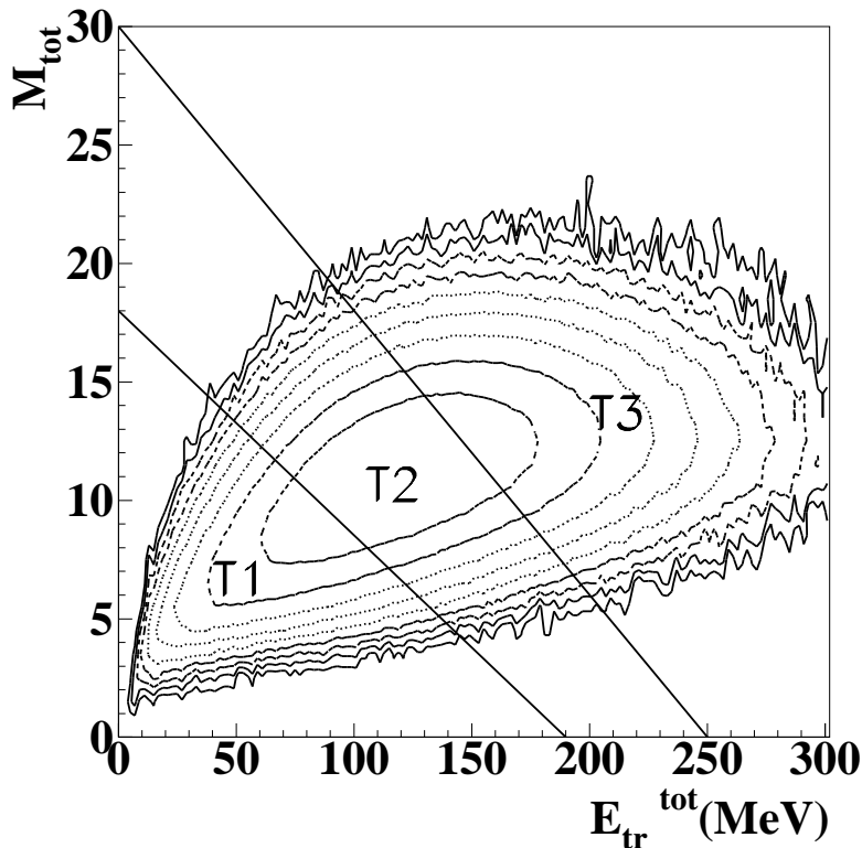
Fig. 2. Total Multiplicity M_{tot} versus Total Transverse Energy E_{tr}^{tot} .
