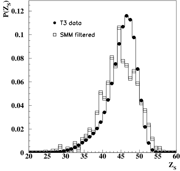
Fig. 9. Source charge distributions : experimental (full points) and SMM backtraced results (open squares) for region T3.
