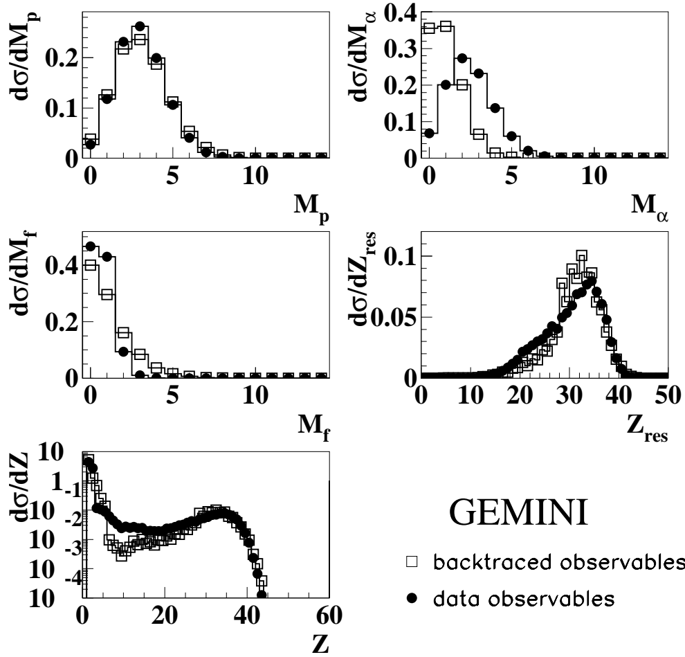
Fig. 5. Comparison between data (full points) and GEMINI results (open squares) for region T3. In the top row : M_p : proton multiplicity and M_\alpha : alpha multiplicity; in the middle row : M_f : fragment multiplicity and the residue charge distribution. In the bottom row : the total charge distribution.
