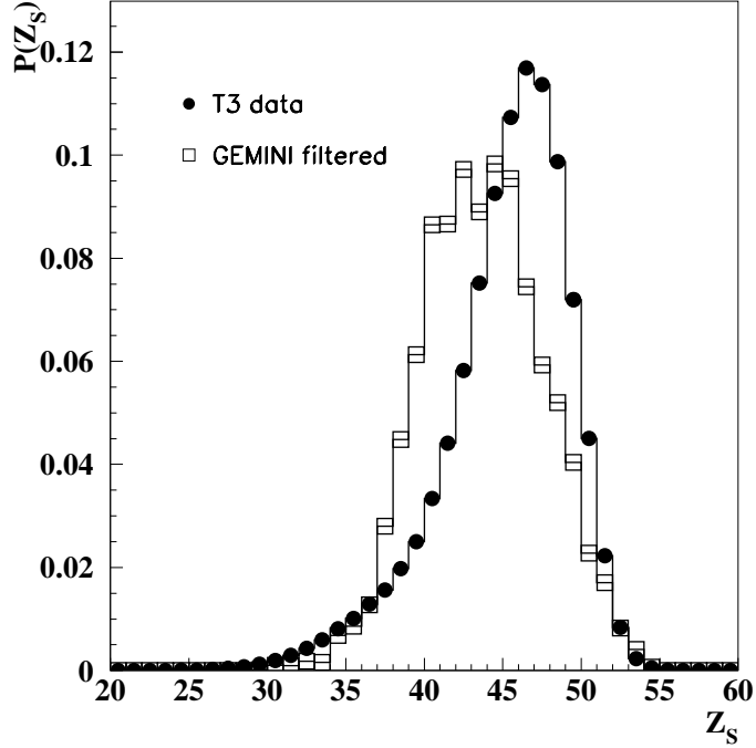
Fig. 6. Source charge distributions : experimental (full points), GEMINI backtraced filtered (open squares) for region T3.
