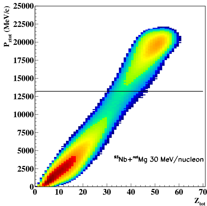
Fig. 1. Total parallel momentum ( P_{z\text{tot}} ) versus total charge ( Z_{\text{tot}} ) for the ^{93}\text{Nb} + ^{\text{nat}}\text{Mg} system at 30 MeV/nucleon.
