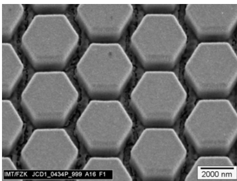
Figure 4b. Detailed view of the honeycomb structures after E-beam lithography. The thickness of the resist is 3 \mu\text{m} .
