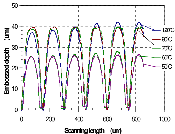
Fig.6. Effect of embossing temperature on patterns in Group A with channel-width/line-width being 50 \mu m/100 \mu m.
