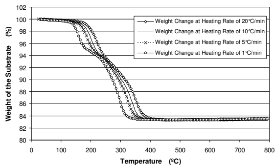
Fig.1. TGA curves of green substrate at different heating rates. The weight loss below 110 °C was attributable to evaporation, and the thermal degradation below 400 °C showed two obvious regions.
