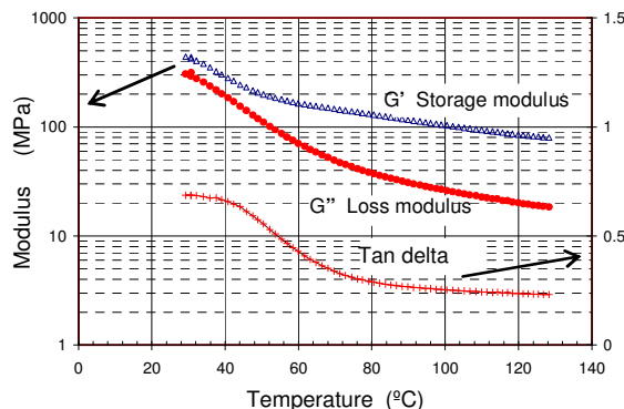
Fig. 2. DMA curves for analyzing glass transition temperature of ceramic green substrate.
