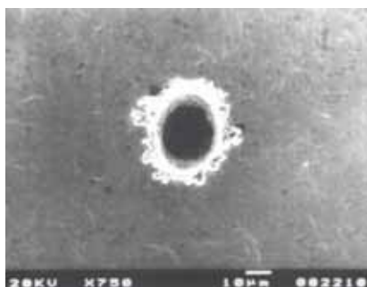
Fig.5 SEM photo of a micro hole machined by a fine electrode of 10µm by EDM machining. The copper plate is 50µm. The current is 0.3A, Voltage is 35V. The machining time is about 1min.
