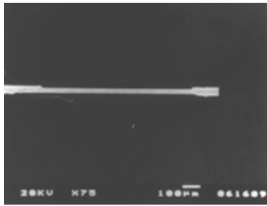
Fig.2 SEM photo of 20µm tungsten carbide microelectrode. This electrode is obtained by 0.5mA and 10V for 1/2hr. The original diameter before machining was 50µm.
