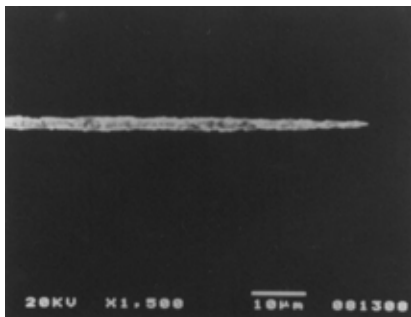
Fig.4 SEM photo of 2µm tungsten carbide. This electrode is obtained by 0.1mA and 10V for 1hr. The original diameter before machining was 20µm.
