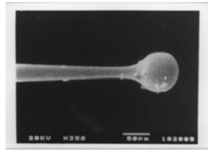
Fig.6 SEM photo of a micro probe by electrolysis. The machined current is 0.2mA, Voltage is 10V. The machine time is about 20min.
