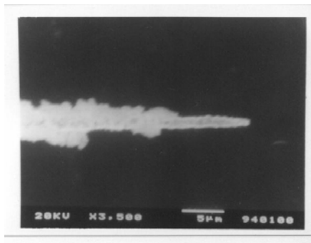
Fig.3 SEM photo of 10µm tungsten carbide. This electrode is obtained by 0.2mA and 10V for 45min. The original diameter before machining was 20µm.
