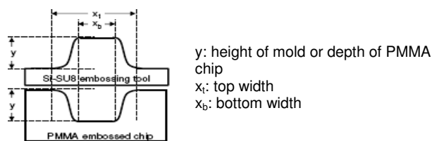
Fig. 3 Channels dimensions measured by mechanical stylus measurements listed in Table 1.
