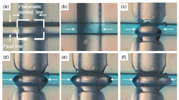
Fig. 7 Micrograph showing pneumatic control of blue electrolytic fluid dye (at a flow rate of 1 μL/min) via a single embedded PDMS based microvalve during (a) no fluid flow, (b) open valving, and valving actuated at (c) P=10kPa, (d) P=14kPa, (e) P=29kPa, and (f) P=34kPa. The top horizontal channel is the PMMA fluid channel while the bottom vertical channel is the pneumatic control line. White arrows in (b) – (f) indicate the location of membrane actuation.
