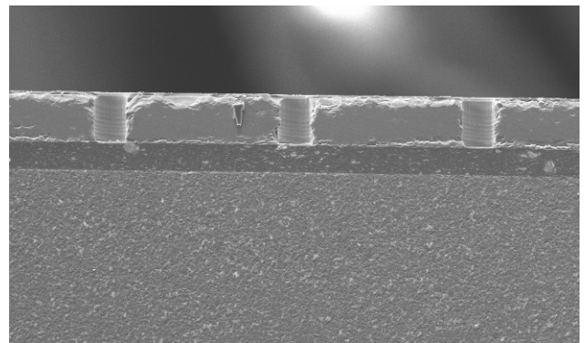
Fig. 3. Cross-sectional view of via holes
