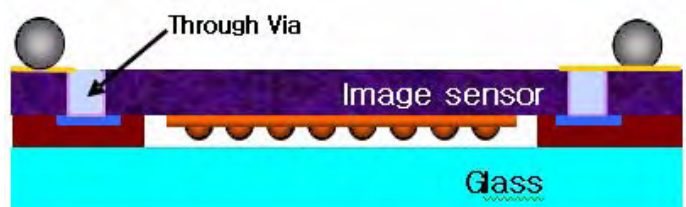
Fig. 1. Structure of ISM WLP with TSV interconnection.
