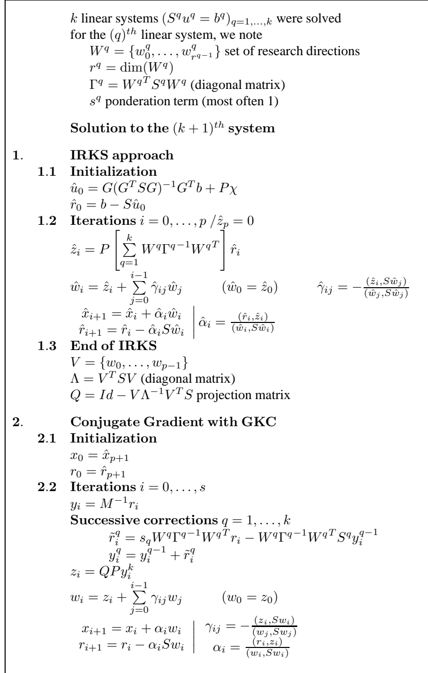
Figure 1. Algorithm: GIRKS with Projected Preconditioned Conjugate Gradient
