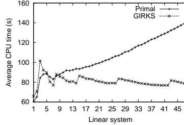
Figure 10. GIRKS: CPU time
