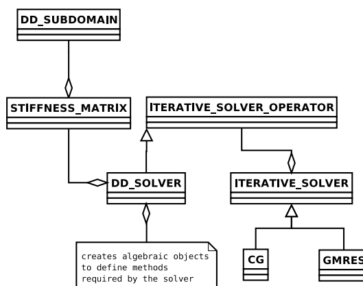
Figure 16. Articulation between formulation and solver
