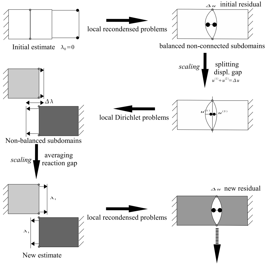
Figure 11. Representation of the first iteration of preconditioned FETIDP
