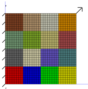
Figure 17. 16 subdomains decomposed square
