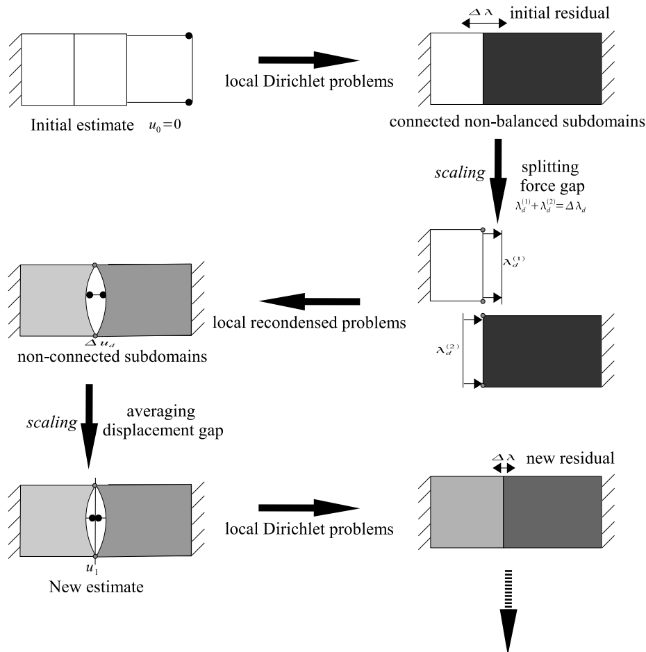
Figure 12. Representation of the first iteration of preconditioned BDDC
