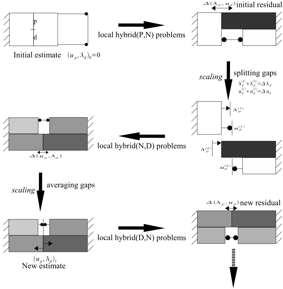
Figure 10. Representation of first iteration of preconditioned hybrid approach
