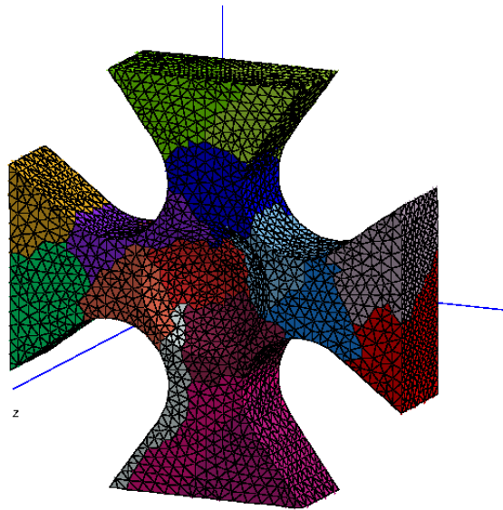
Figure 2. 16 subdomains bitraction test specimen (courtesy of ONERA – Pascale Kanouté)
