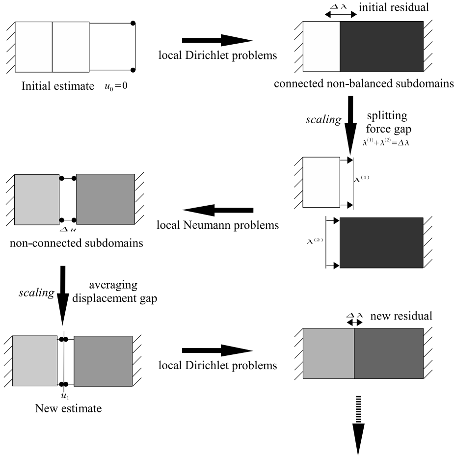
Figure 8. Representation of first iteration of preconditioned primal approach
