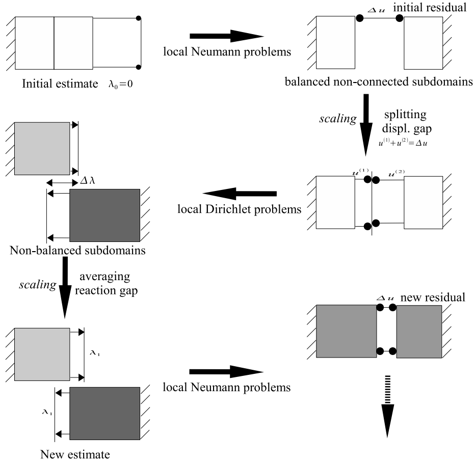
Figure 9. Representation of first iteration of preconditioned dual approach
