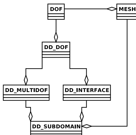
Figure 14. Topological interface information
