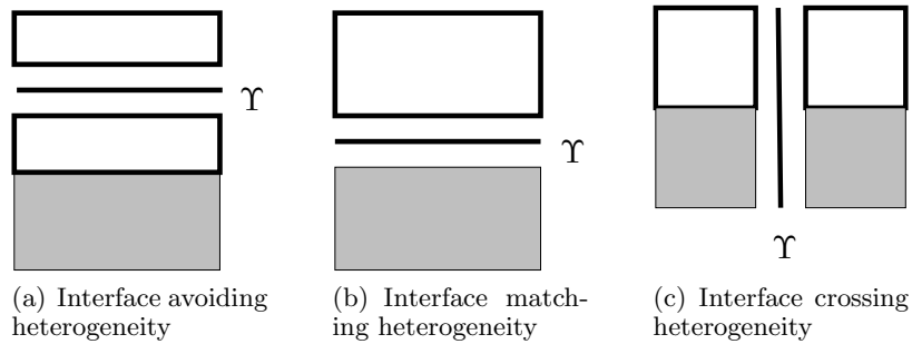
Figure 13. Different kinds of heterogeneity in domain decomposition context
