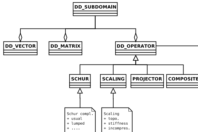
Figure 15. Algebraic interface objects
