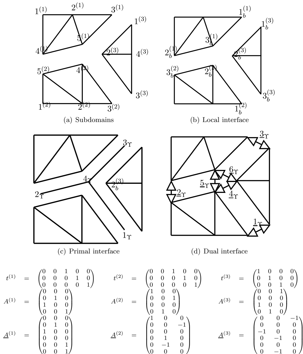
Figure 6. Local numberings, interface numberings, trace and assembly operators
