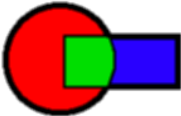
Figure 1. Schwarz' original problem
