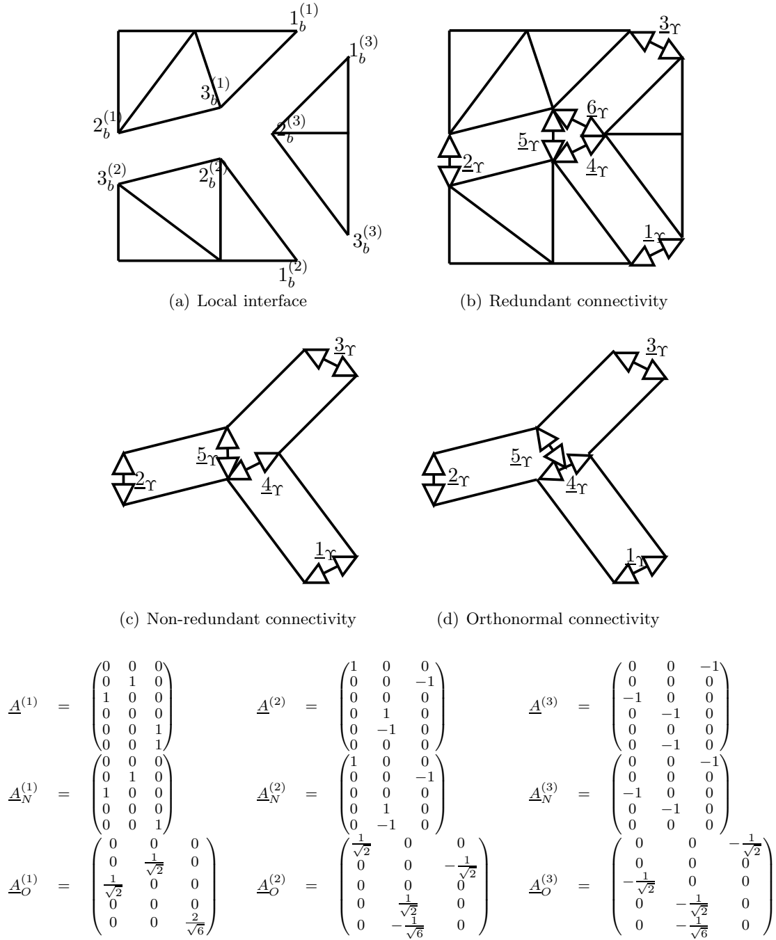
Figure 7. Suppressing redundancies of dual interface
