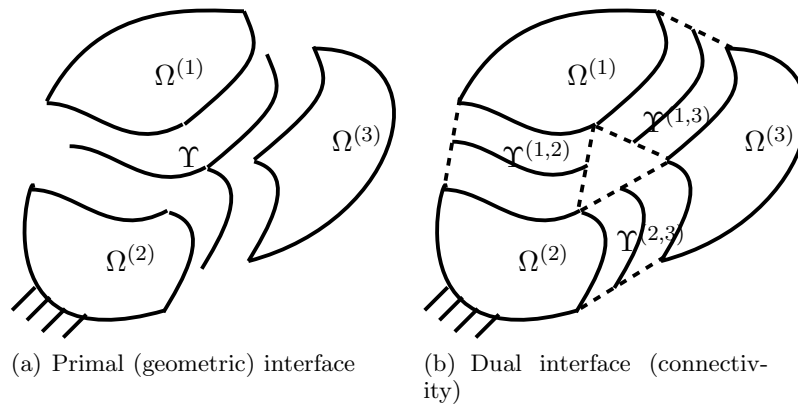
Figure 5. Definition of the interface for a N -subdomain decomposition
