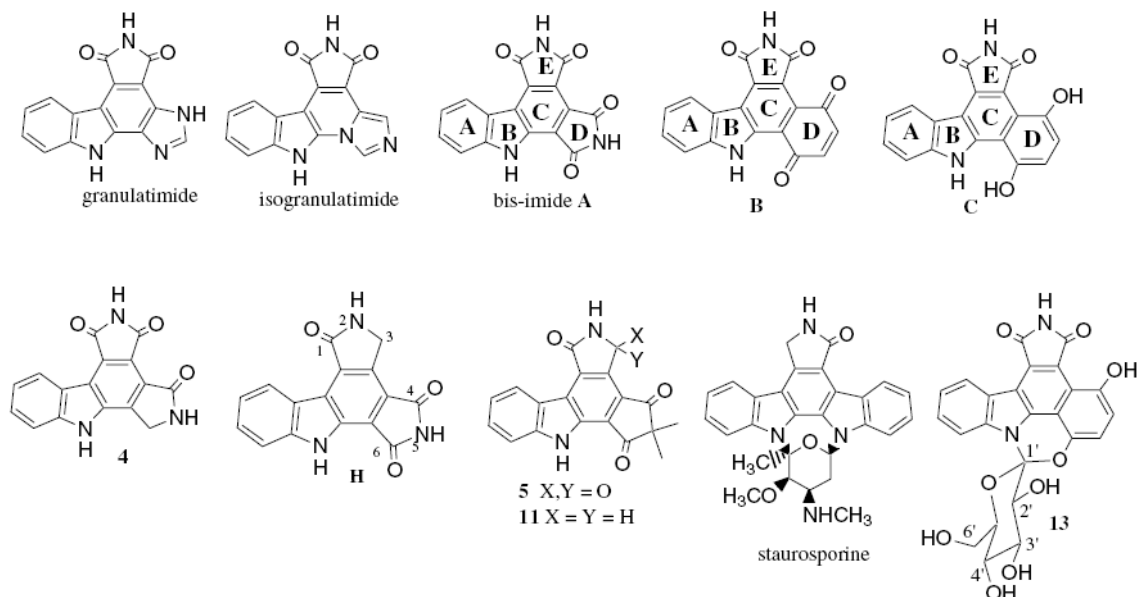
Figure 1. Chemical structures of granulatinamide, isogranulatinamide, staurosporine, compounds A, B, C, and H previously described and newly synthesized compounds 4, 5, 11, and 13.
