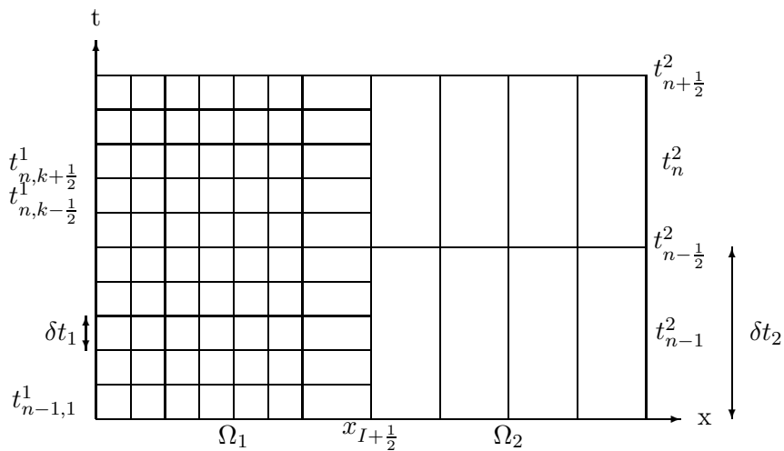
Figure 2: Time-space discretization.
