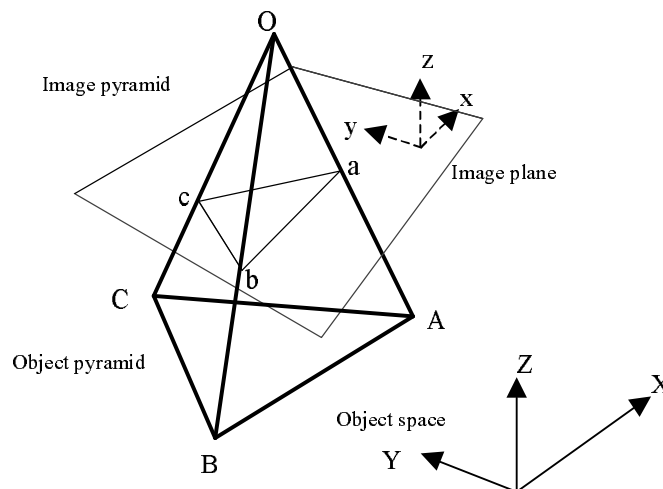
FIG. 2. Space resection
