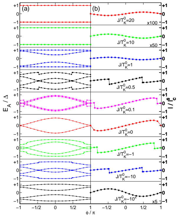
FIG. 2: (color online) (a) ALs in units of \Delta and (b) supercurrents I in units of I_c^s \equiv e\Delta/\hbar as functions of \phi in the strong coupling limit ( \Delta/T_K^0 = 0.1 ) for various values of J/T_K^0 : see the line aa' in Fig. 1. Here the ion spin S is set to 1/2 .
