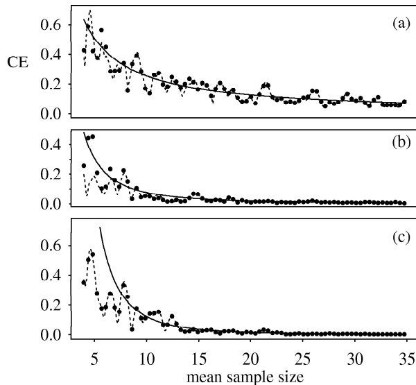
Figure 4: Coefficients of error for Cavalieri volume estimators. Exact coefficients of error (CE) calculated from simulations are represented by dots. Approximated CE based on primary transitions are represented by dashed line curves, cf. (5). Approximated CE based on primary transition amplitudes (extension term) are represented by solid line curves, cf. (9). Underlying structures are described in Section 2.
