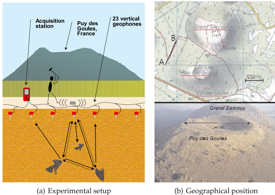
Figure 2.9. (a) Seismic source in the middle of an array of geophones. Solid and dashed arrows illustrate reciprocal scattered wave paths. (b) Map and picture of the volcano. The line AB marks the position of the array. Map from IGN.
