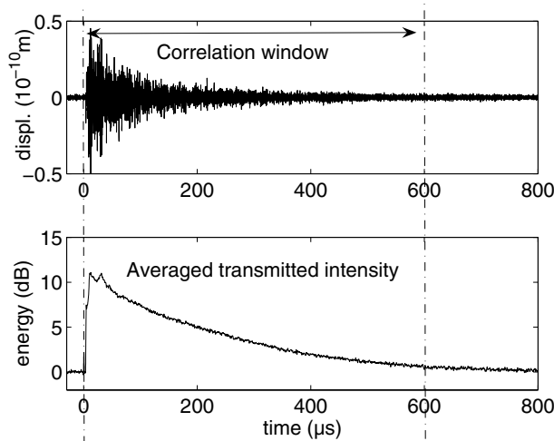
Figure 4.11. Top: typical waveform obtained through the scattering slab around 1 MHz. The sensitivity of the heterodyne interferometer is 10^{-4} \text{ \AA} / \sqrt{\text{Hz}} corresponding the optimal level of optical reflection on the sensed surface. After averaging over 100 records we reached the precision of 10^{-2} \text{ \AA} . Bottom: intensity averaged over several source/sensor positions. Figure reprinted with permission from [É. Larose et al. , Phys. Rev. E 72 , 046607 (2005)]. Copyright 2007 by the American Physical Society.
