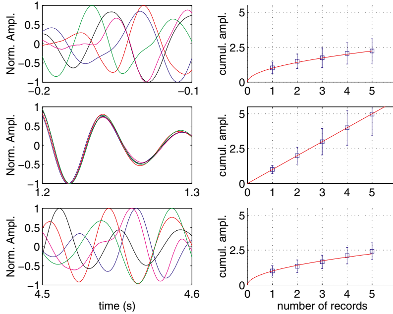
Figure 2.11. Top: incoherent summation of human noise. Middle: coherent summation of the seismic response. Bottom: incoherent summation of ambient background noise. Each record is made of N = 10 strikes.
