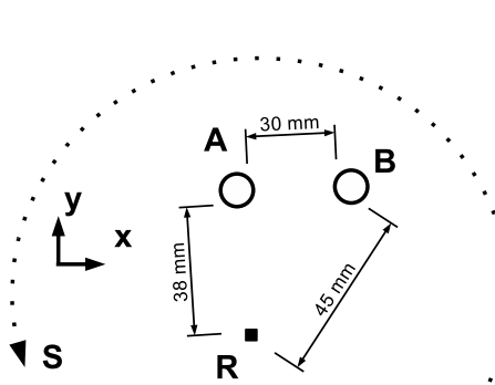
Figure 3.8. Sketch of the first experiment. A source S sends a broadband pulse s(t) in an open medium. It is sensed by a fixed omnidirectional receiver R . Two 8 mm-diameter empty cylinders are placed nearby (approximate distances displayed). The source is rotated all over the setup for 2000 different positions, along a perfect circle of radius 80 mm. Figure reprinted with permission from [É. Larose et al. , Appl. Phys. Lett. 88 , 104103 (2006)]. Copyright 2007, American Institute of Physics.
