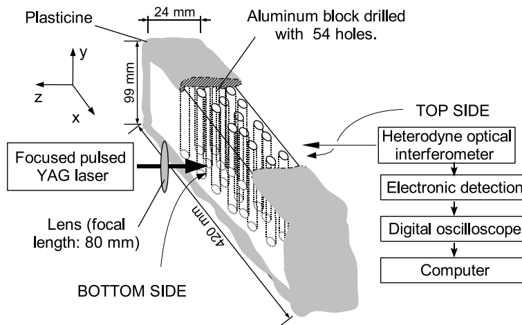
Figure 4.10. Experimental setup: the propagation medium is an aluminum block drilled with 54 vertical cylindrical holes (diameter: 4 mm). A Q-switched Nd:YAG laser shoots on the bottom side 100 pulses (24 ns duration and 280 \text{ MW}/\text{cm}^2 intensity each). On the top side a heterodyne interferometer senses the vertical displacement of the aluminum/air interface. This measure is repeated at 7 different locations ( X_0 = 0 \text{ mm} \rightarrow X_6 = 60 \text{ mm} ) for each source position. Plasticine was stuck on the edges and the four lateral sides to mimic absorbing boundary conditions and avoid the generation of Rayleigh waves by mode conversion at the edges. Figure reprinted with permission from [É. Larose et al. , Phys. Rev. E 72, 046607 (2005)]. Copyright 2007 by the American Physical Society.
