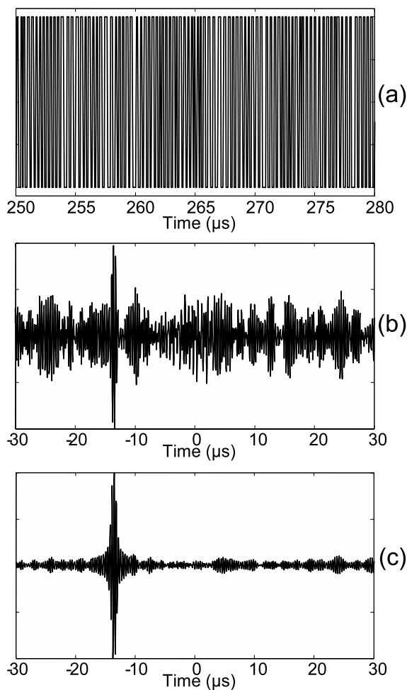
Figure 5.4. Same as Figure 5.2, except that only the sign (+1/−1) of the scattered wave forms has been recorded and cross correlated (one-bit correlations). Figure reprinted with permission from [É. Larose et al. , J. Appl. Phys. 95 , 8393 (2004)]. Copyright 2007, American Institute of Physics.
