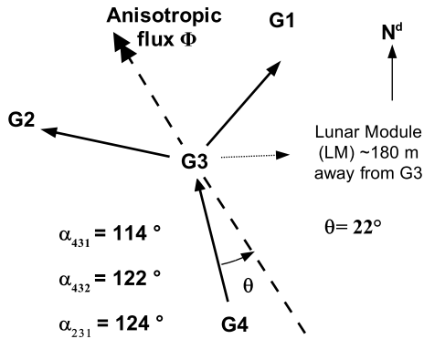
Figure 5.15. Schematic view of the anisotropic flux.
