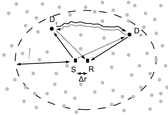
Figure 2.8. Schematic view of the propagation of waves from the source \mathbf{S} to the receiver \mathbf{R} . Dashed line is for reciprocal paths. If the source-sensor distance \Delta r is smaller than the wavelength, reciprocal paths interfere constructively. Crawling arrows are for the intensity diffusion between the first and the last scatterer.
