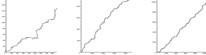
FIGURE 6. Random 2-sided walks of length 500, 1354 and 3148.
