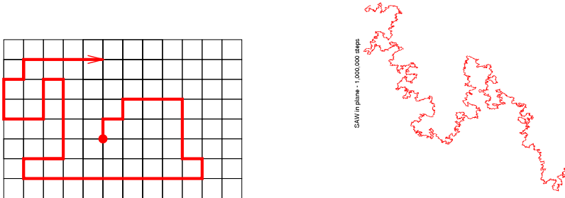
FIGURE 1. A self-avoiding walk on the square lattice, and a (quasi-)random SAW of length 1,000,000, constructed by Kennedy using a pivot algorithm [19].
