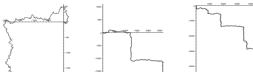
FIGURE 13. Kinetic prudent walks with 1000, 10000 and 20000 steps.
