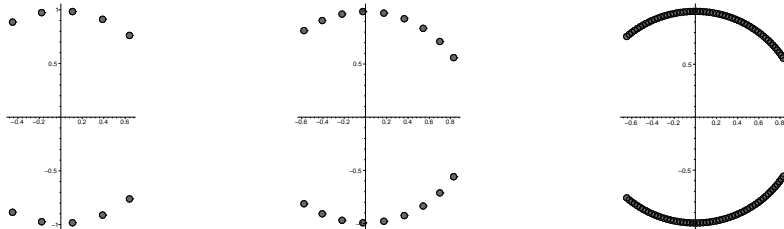
FIGURE 9. The roots of Y(t)t^\ell(1 - 2t^2) = 1 lying inside the domain \mathcal{D} for \ell = 20 , \ell = 30 , \ell = 200 .
