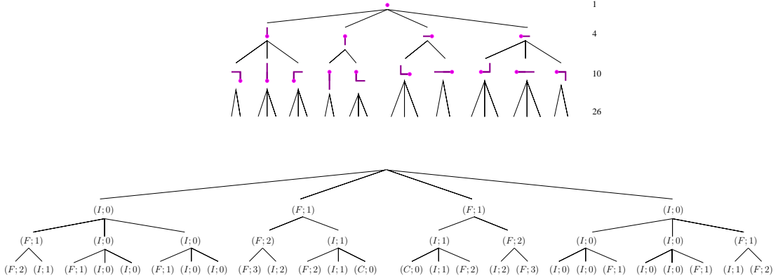
FIGURE 12. The generating tree of 2-sided walks (top) and one of its good labellings (bottom).
