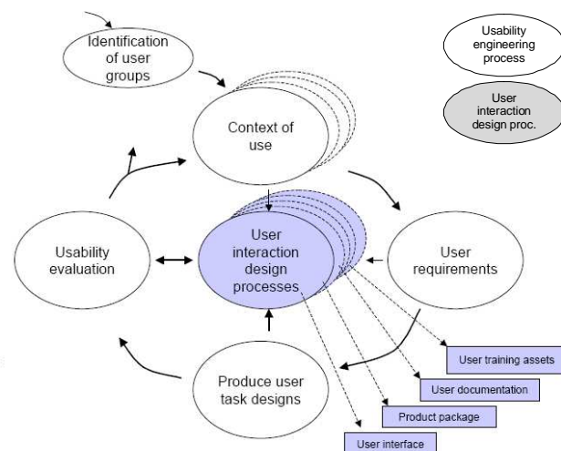
Figure 2 Jokela’s UCD Process Model
