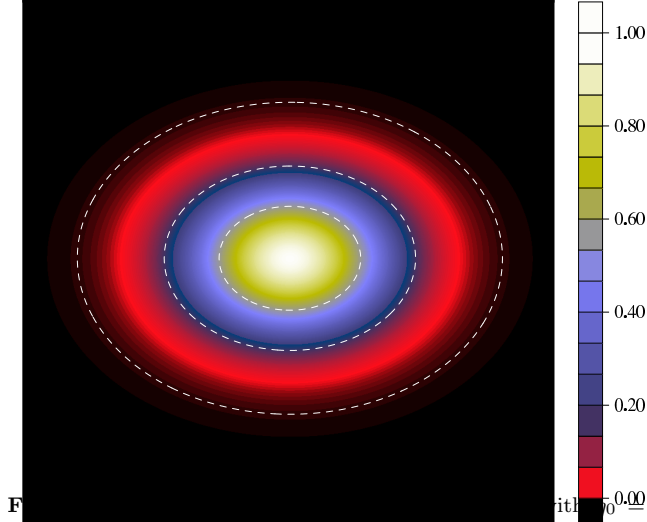
Figure 2. The three dashed lines correspond to isophotes defined by I(R_1) = 0.6 I_{\max} , I(R_2) = 0.2 I_{\max} and I(R_3) = 0.01 I_{\max} .
