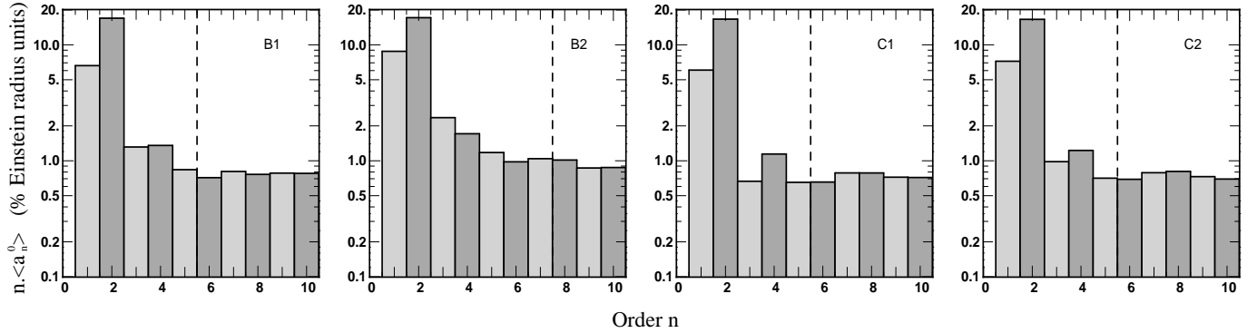
Figure 10. Variation of mean amplitudes n \times \langle a_n^0 \rangle for each lenses catalogue. The dashed line represents the confident limit.
