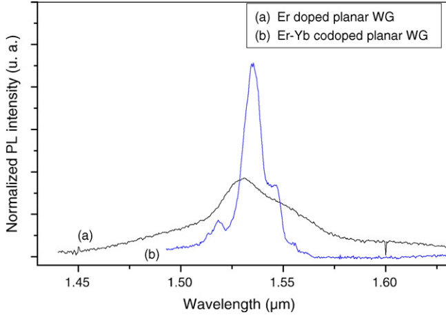
Fig. 2. Room temperature photoluminescence spectra relative to the ^4I_{13/2} \rightarrow ^4I_{15/2} transition of Er^{3+} for erbium doped porous silicon waveguide (a) and Er-Yb co-doped porous silicon waveguide (b) after thermal treatments with excitation pump powers at 488 nm.
