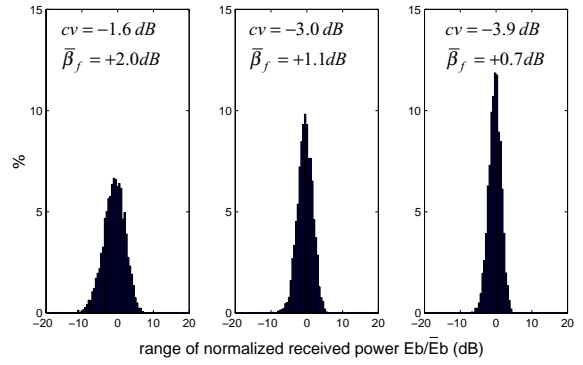
Fig. 12.- Vehicular B performances with fading. Performances en Vehicular B avec fading.
