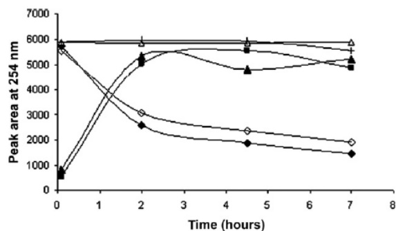
Fig. 1. Release of compound 1a' from 1a catalyzed by TK. Controls: 1a (100 \mu\text{M} ), TK extract (1 unit \text{mL}^{-1} ); \Delta : 1a in Bicine buffer pH 8.2; +: 1a in Mops buffer pH 7.2. Reactions: 1a (100 \mu\text{M} ), D-ribose-5-phosphate (100 \mu\text{M} ), TK extract (1 unit \text{mL}^{-1} ); \diamond : 1a , \blacktriangle : 1a' in Bicine buffer 0.1 M pH 8.2; \blacklozenge : 1a , \blacksquare : 1a' in Mops buffer 0.1M pH 7.2.
