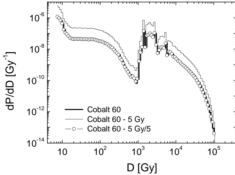
Figure 6: Histogram of local dose calculated for a sample of 10 \times 10 \times 10 \text{ }\mu\text{m}^3 irradiated with a dose of 1 Gray and 5 Grays of ^{60}\text{Co} \gamma rays. The mesh resolution is 10 nm. The curve labeled with “Cobalt 60-5Gy/5” represents the histogram calculated for 5 Grays and divided by a factor 5.
