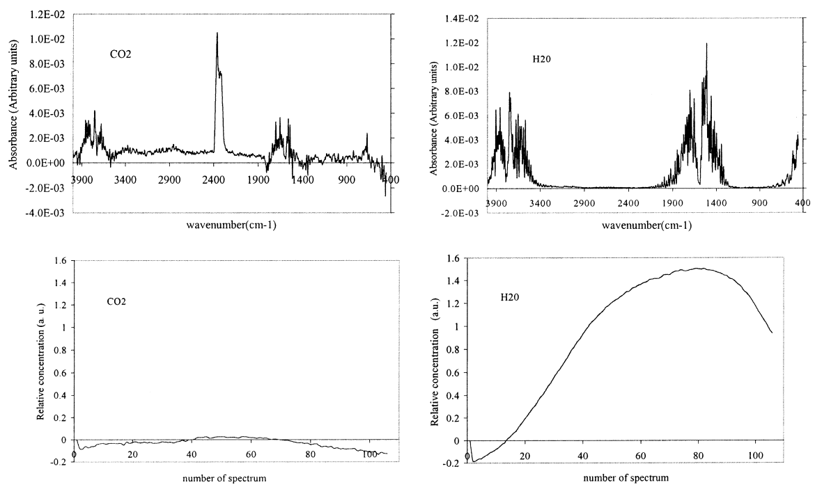
Fig. 3. Resolved spectra and relative contributions from zone I.
