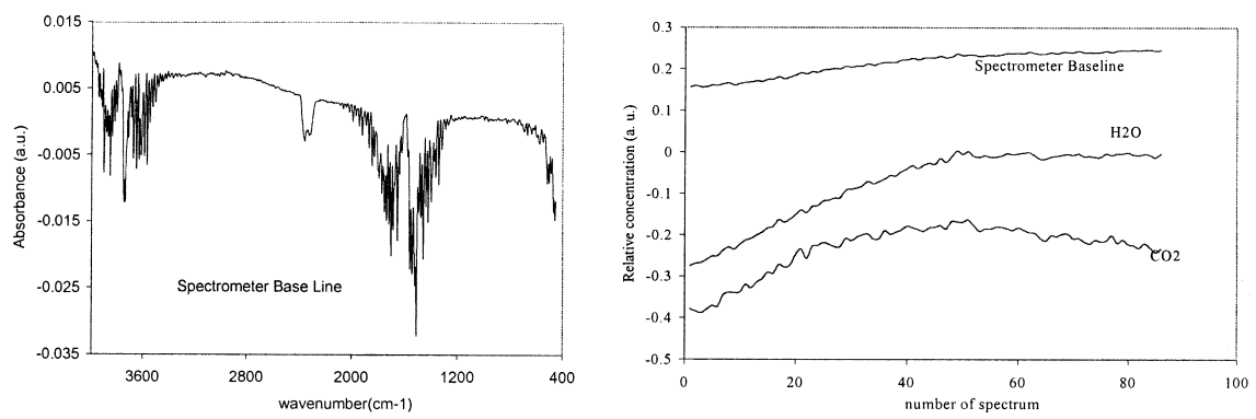
Fig. 5. Relative contribution profiles from zone III.
