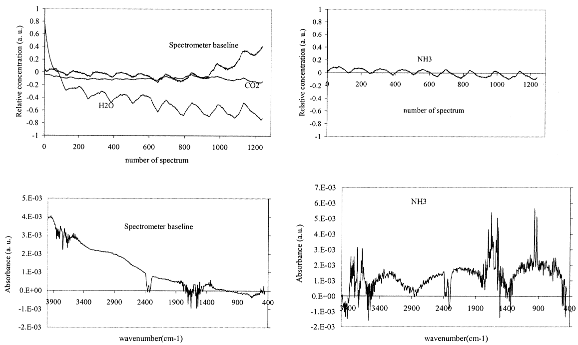
Fig. 4. Resolved spectra and relative concentration profiles from zone II.
