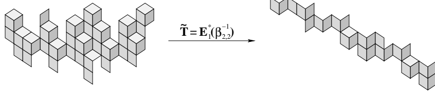
Fig. 8. The recognizable binary function \mathcal{B} of Fig. 6 is transformed by applying the rules of Fig. 7 into a binary function \tilde{\mathcal{B}} (left) such that 0 \leq \mathcal{B} \leq \mathcal{P} \Leftrightarrow 0 \leq \tilde{\mathcal{B}} \leq \mathcal{P} . Here, since \tilde{\mathcal{B}} does not have open (1, 3) -run, its image by \tilde{T} (right) is such that, for any stepped plane \mathcal{P} , one has: 0 \leq \tilde{\mathcal{B}} \leq \mathcal{P} \Leftrightarrow 0 \leq \tilde{T}(\tilde{\mathcal{B}}) \leq \mathcal{P} .
