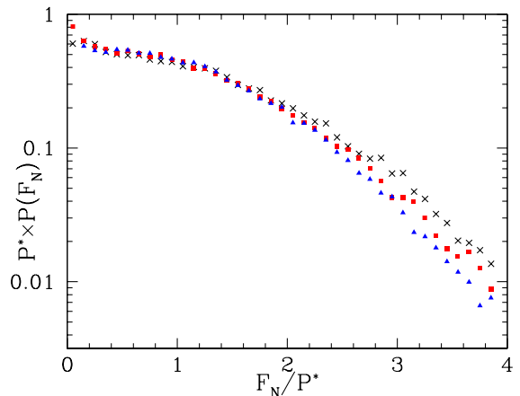
FIG. 19: (Color online) Positive wing of probability distribution function of rescaled normal forces, F_N/P^* , in systems with no RR, under P^* = 2.37 (black crosses), P^* = 5.62 (red square dots), P^* = 13.3 (blue triangles).
