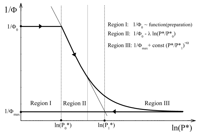
FIG. 10: Schematic view of intrinsic consolidation curve with regimes II and III, and role of parameters introduced in Eq. (9).
