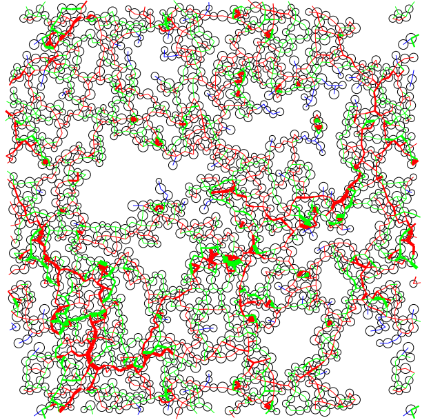
FIG. 2: (Color online) Equilibrium configuration of a sample of 1400 disks with RR in initial state, under P^* = 0.01 , for which \Phi = 0.5132 . Line thicknesses encode normal force intensities, red strokes depict compressive forces while tensile ones are colored in green, and forces equal to zero in blue.
