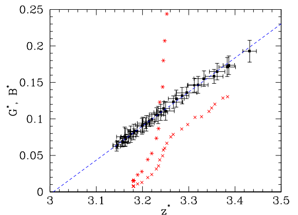
FIG. 23: (Color online) Elastic moduli (no RR) divided by \Phi(1 - x_0) , versus z^* . We recall that z^* is the coordination number without rattlers. Data with error bars correspond to G in cohesionless systems, for which the dashed line is a linear fit. G and B in the cohesive material are respectively shown as (red) crosses and asterisks.
