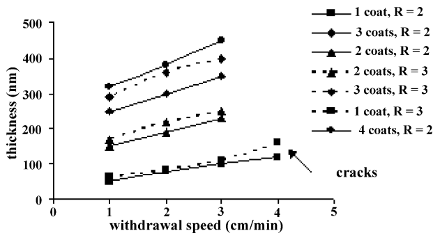
Fig. 6. Evolution of the thickness of La 2 NiO 4+δ multilayers prepared with R=2 and 3 as a function of the withdrawal speed and the number of coats.
