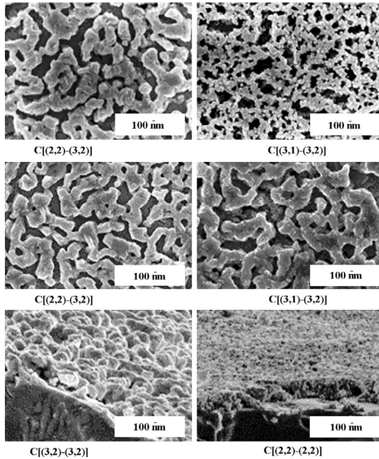
Fig. 3. SEM-FEG micrographs of \text{La}_2\text{NiO}_{4+\delta} bilayers: \text{C}[(2,2)-(2,2)] , \text{C}[(3,2)-(3,2)] , \text{C}[(2,2)-(3,2)] , \text{C}[(3,2)-(2,2)] ; cross-section of interlayers \text{C}[(2,2)-(2,2)] and \text{C}[(3,2)-(3,2)] .
