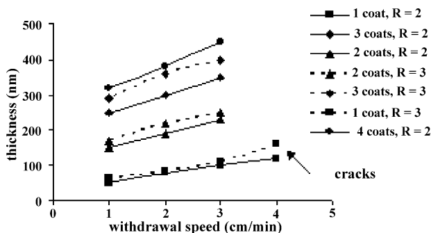
Fig. 6. Evolution of the thickness of \text{La}_2\text{NiO}_{4+\delta} multilayers prepared with R=2 and 3 as a function of the withdrawal speed and the number of coats.
