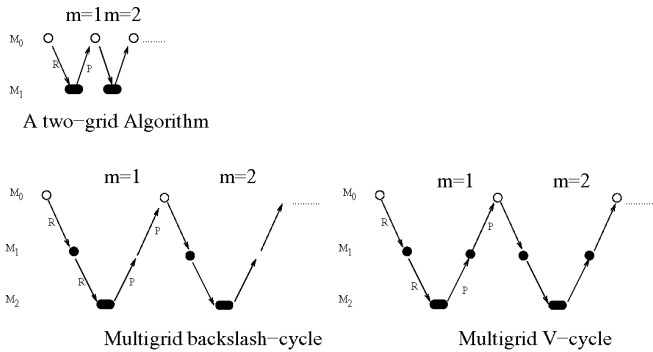
Figure 3 Multigrid cycles
