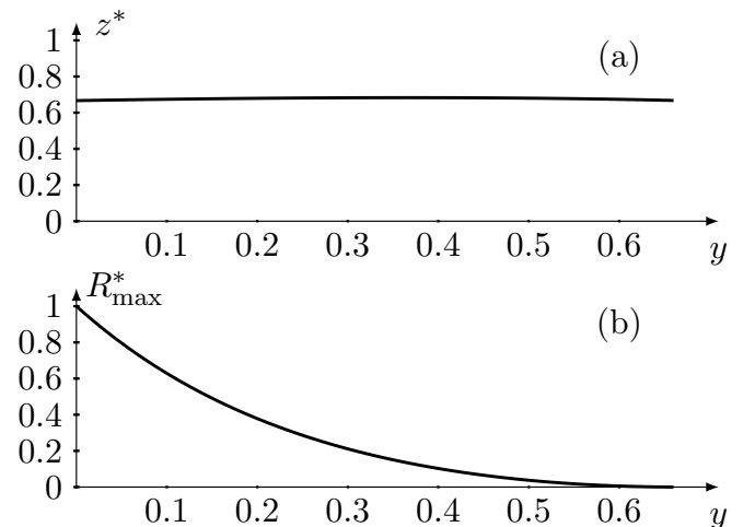
FIG. 3: (a) The optimal mirror velocity z^*(y) = V^*/v_i normalized to v_i is plotted as a function of the dimensionless parameter y = \Delta v/v_i and (b) the corresponding maximum phase space density R_{\max}^* = R_{\max}(y, z^*(y)) = \rho'/\rho_p of a beam generated from the packet after their optimal slowing down and normalized to the packet initial phase space density, is plotted as a function of y .
