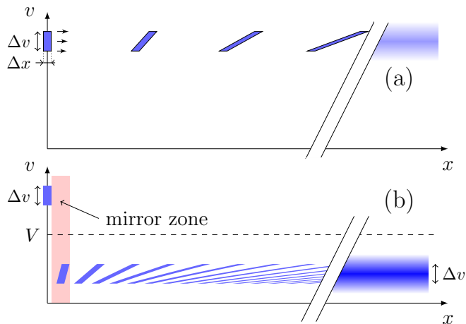
FIG. 2: (Color online) Representation in the single-particle phase space of one-dimensional atomic packets periodically injected in a guide. a) in the absence of slowing b) in the presence of slowing with the mirror moving at a velocity V (dashed line). For a sufficiently long propagation distance, packets have merged and the thermal equilibrium for the corresponding beam is reached.
