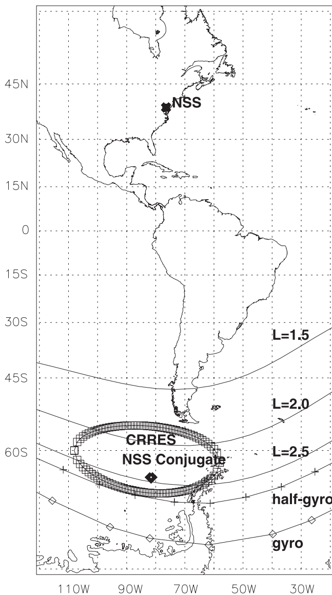
Figure 7. A map of the location of the region of large intensity signals from the NSS transmitter in Washington, USA. The circle represents signal intensities >10^{-5} \text{mV}^2 \text{m}^{-2} \text{Hz}^{-1} . Only observations made at the equatorial plane of the magnetic field line (dashed line) are shown as NSS stopped operating before DEMETER became operational.
