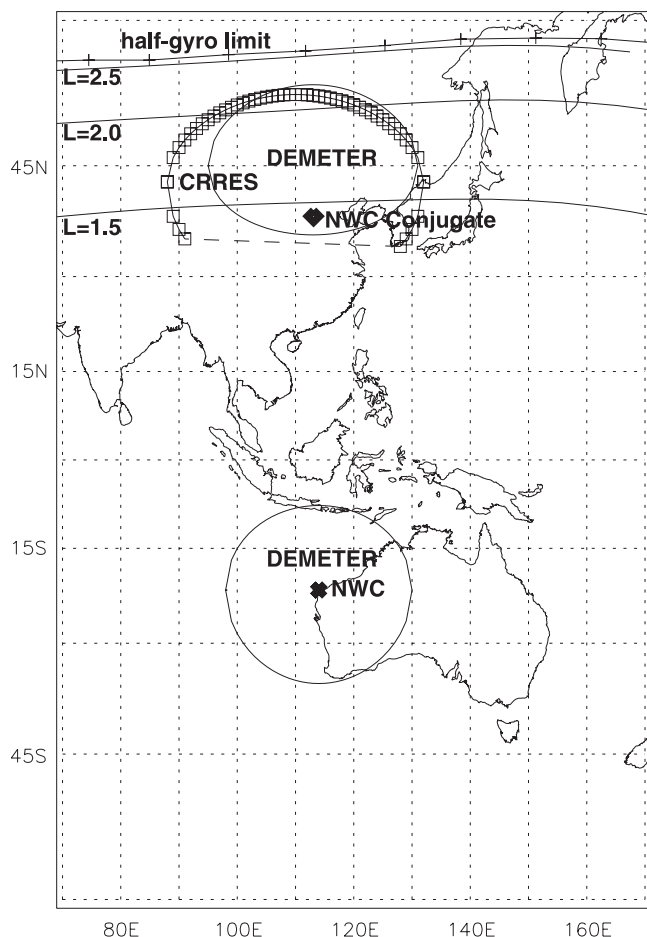
Figure 2. A map of the locations of the regions of large intensity signals from the NWC transmitter in Australia. The circles represent signal intensities >3 \times 10^2 \mu\text{V}^2 \text{m}^{-2} \text{Hz}^{-1} for DEMETER and >10^1 \mu\text{V}^2 \text{m}^{-2} \text{Hz}^{-1} for CRRES. Observations made by DEMETER at 700 km above the transmitter (solid line), by CRRES at the equatorial plane of the magnetic field line (squares), and by DEMETER at 700 km altitude in the conjugate region (solid line) are shown, using the results from Figure 1. Contours for L = 1.5 , 2.0 , 2.5 , and the electron half-gyrofrequency cutoff for 19.8 kHz ducted waves are also plotted.
