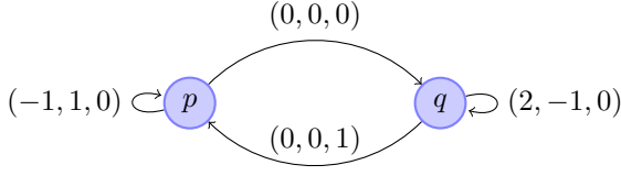
Figure 2. A VASS taken from [5].
