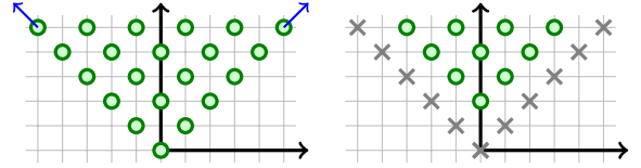
Figure 4. On the left a monoid M . On the right its interior \mathcal{I}(M) .
