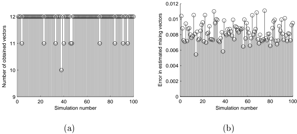
Fig. 7. Efficiency of the overall algorithm for all simulations in the case n = 12 , m = 6 , k = 2 and T = 3900 for 100 different simulations. In (a) number of obtained vectors in each simulation is shown. In some cases fewer than 12 vectors are obtained and type one error has occurred. In (b) error in obtaining the mixing vectors is measured using (9). Negligible errors show type two error has never occurred.
