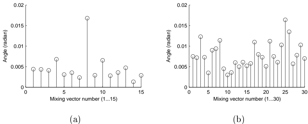
Fig. 8. The angle (in radian) between the mixing vectors and their corresponding estimation in middle scale problems. In (a) n = 15 , m = 7 and k = 3 . In (b) n = 30 , m = 15 and k = 2 .
