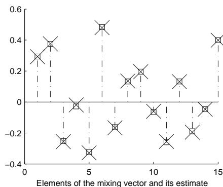
Fig. 9. Comparison between the most erroneous obtained vector and its corresponding mixing vector, for the second case ( n = 30 , m = 15 and k = 2 ) in experiment 2. The crosses show the values of elements of the obtained vector and the squares show their actual values.
