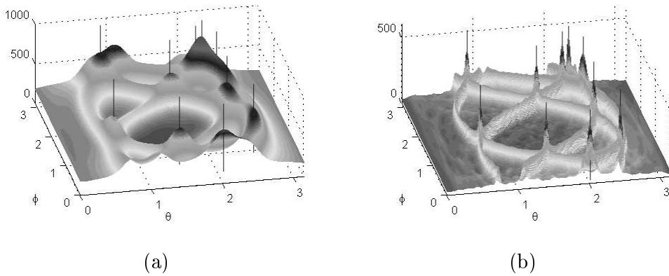
Fig. 4. Graph of the function f in the case n = 5 , m = 3 and k = 2 for two different values of \sigma . In (a) \sigma = 0.1 and in (b) \sigma = 0.02 . The exact location of the actual concentration subspaces are indicated by vertical lines. Similar to Fig. 2, by decreasing \sigma , discrimination increases while a decrease in smoothness is observed.
