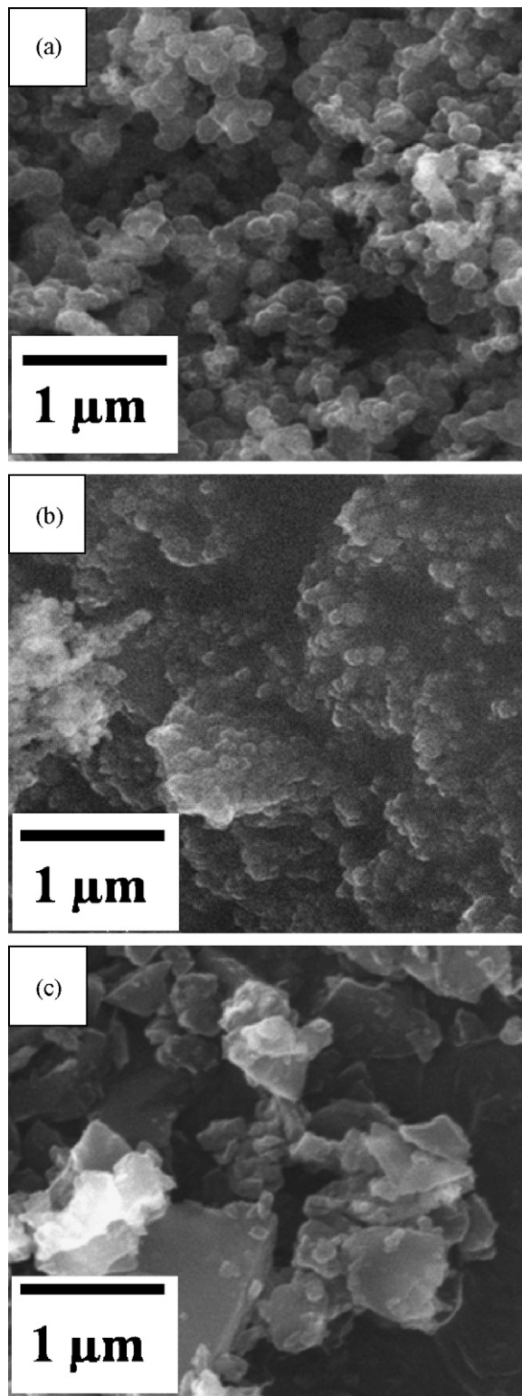
Fig. 3. SEM observations of the starting powders: carbon lampblack (a), boron (b) and boron carbide: B 4 C (c).
