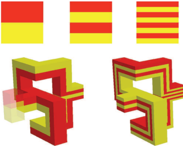
FIG. 1. (Color online) Top: baker's transformation of the unit square after two iterations. Bottom: sketch of mixing action of the present flow after two elements.
