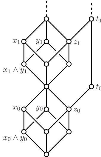
FIGURE 1. The lattice K' .
