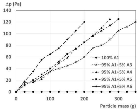
Figure 1: Evolution of pressure drop due to foulant only across a fouled exchanger as a function of the total mass of particles introduced for different size mixtures. Exchanger A; air speed 5 m/s. Dashed lines are included as a visual aid only.
