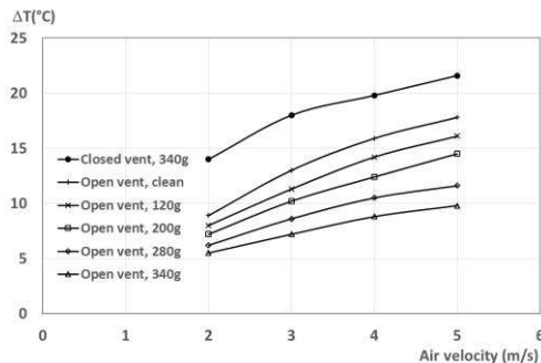
Figure 8: Temperature drop across increasingly fouled exchanger in an open vent wind tunnel as a function of mean air flow velocity.
