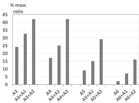
Figure 5: Ratio of the mass of larger particles in the sub-surface region to the total mass of particles introduced for different mixtures. (Exchanger A).
