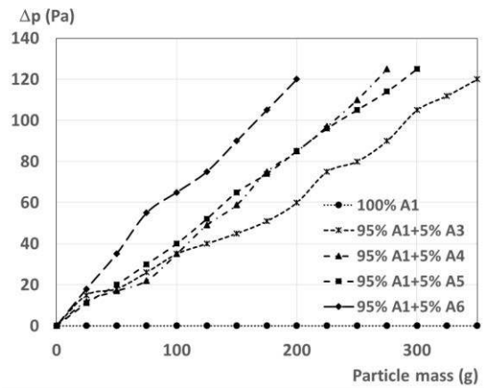
Figure 1: Evolution of pressure drop due to foulant only across a fouled exchanger as a function of the total mass of particles introduced for different size mixtures. Exchanger A; air speed 5 m/s. Dashed lines are included as a visual aid only.
