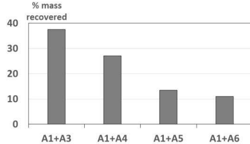
Figure 3: Evolution of the proportion of A1 size particles captured in the sub-surface region as a function of different mixtures.
