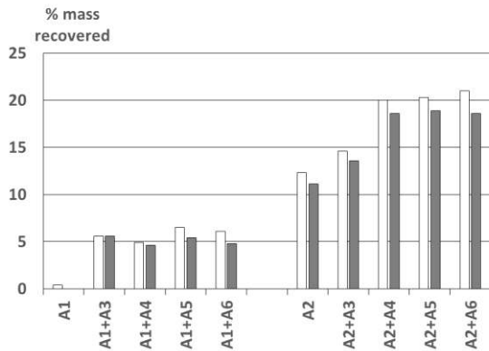
Figure 2a: Ratio of the mass of blocked particles recovered (floor, outer surface and sub-surface) (white) and fouling particles (outer surface and sub-surface) to the total mass of particles introduced into the air stream for different binary mixtures (exchanger A).
