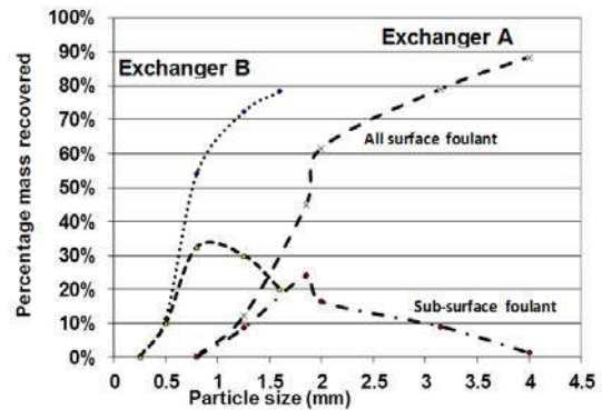
Figure 6: Evolution of the mass of foulant recovered on the exchanger surface as a function of particle size for discrete size ranges. Taken from Haghigi-Khoshkhoo & McCluskey 2007 with kind permission.
