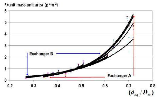
Figure 7: Variation of the fouling factor per unit mass and unit exchanger surface area as a function of non-dimensional equivalent particle size for all binary mixtures of particles examined in both exchangers. (Air speed is 5m/s).
