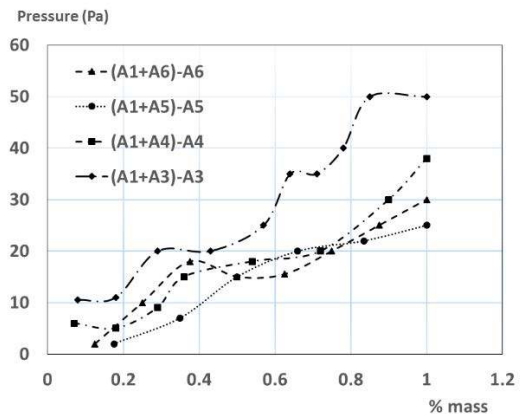
Figure 4: Evolution of the pressure drop across the exchanger due to A1 size particles in different mixtures as a function of increasing mass (divided by the total mass) of particles introduced. Dashed lines are included as a visual aid only.
