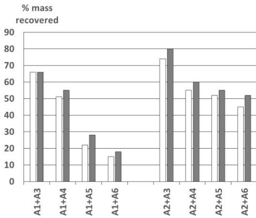
Figure 2b: Ratio of the mass of recovered sub-surface foulant to the mass of blocked (white) and fouling particles (grey) for different binary mixtures (exchanger A).
